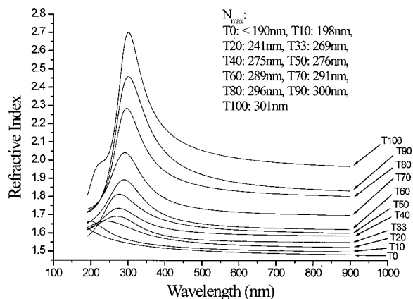
Figure 6. Variation of the refractive indices ( n ) of the hybrid films T0 – T100 in the wavelength range of 190–900 nm.
